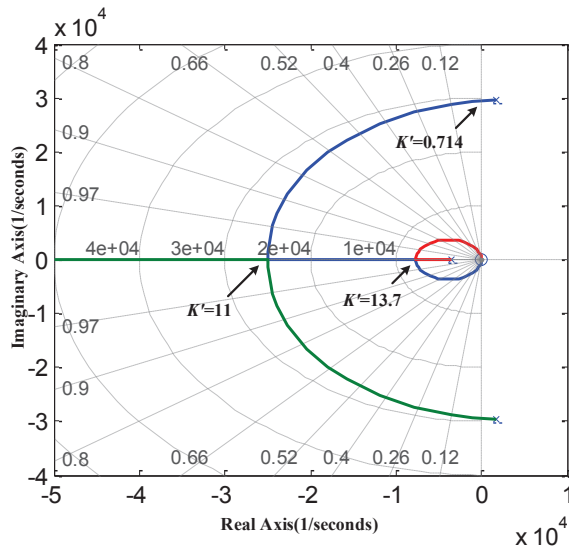
Fig. 12. The generalized root locus of (12) with different K'
