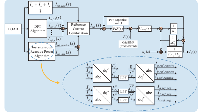
Fig. 2. Control diagram of modular SAPF
