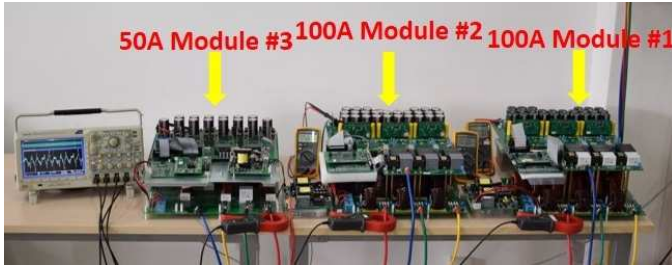
Fig. 15. Hybrid modular three-level SAPF prototype
