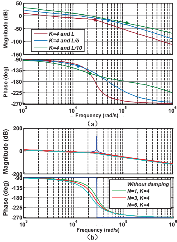
Fig. 9. (a)Frequency characteristics with different output current (b)Frequency characteristics with different number of parallel units
