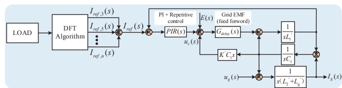
Fig. 11. Novel self-adaptive active damping strategy
