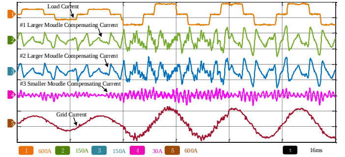
Fig. 18. Compensating current of hybrid modules with load change
