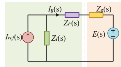
Fig. 3. The proposed single SAPF model in this paper
