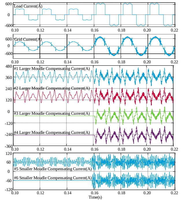
Fig. 14. Simulation results of parallel units increase with six SAPF in parallel operation
