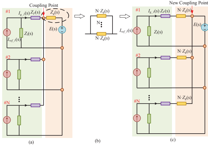
Fig. 6. Modeling of modular SAPF
